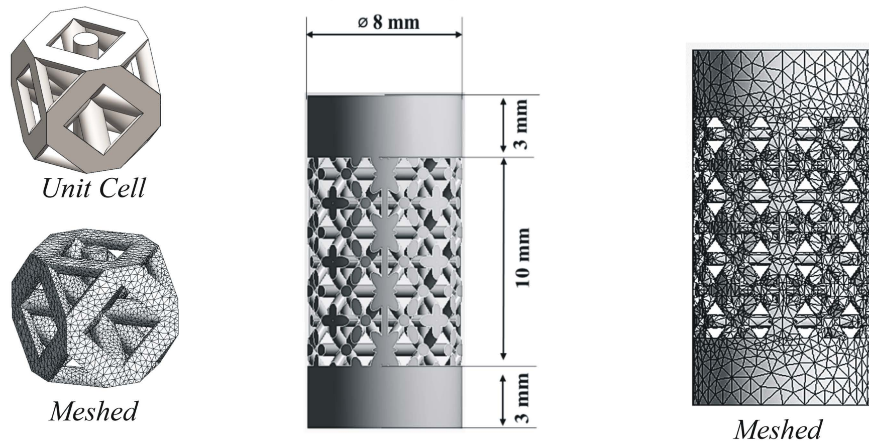
Figure 1: Unit cell and nomenclature of EBM sample
