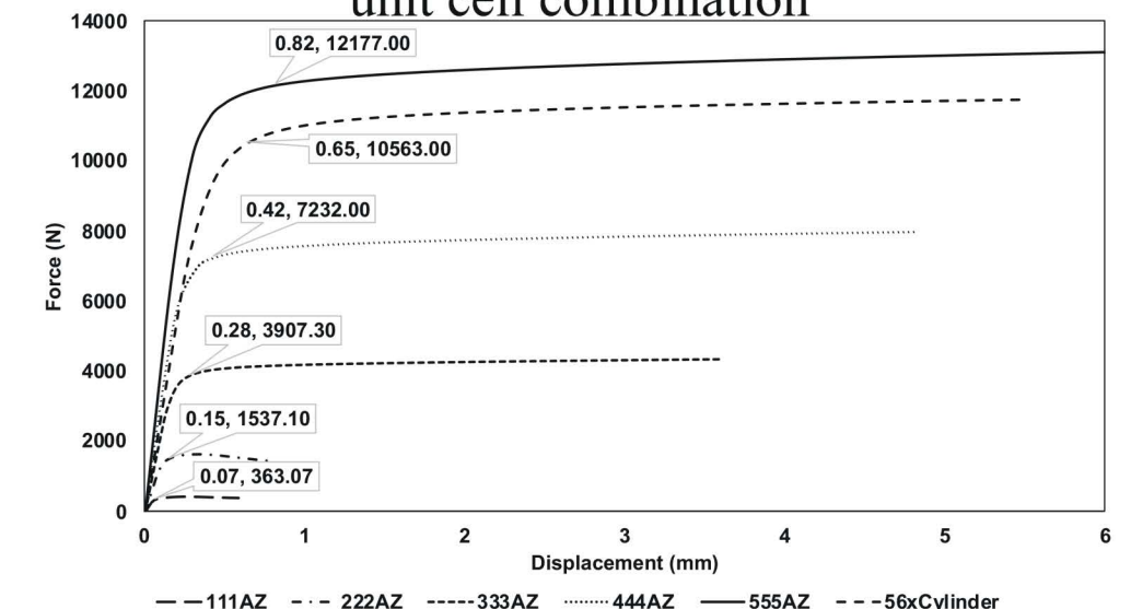
Figure 7: Force vs Displacement graph for each set of unit cell combination
